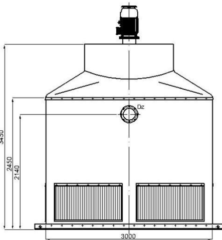
CWT 150/600/BZ
